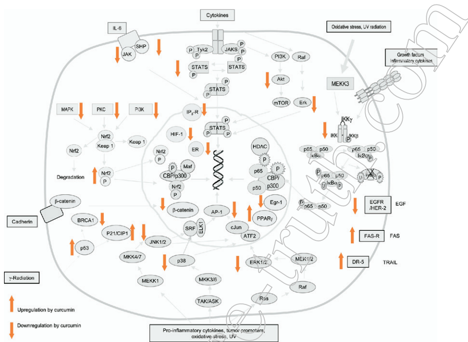
FIG 1. Targets of curcumin. Abbreviations: MEKK, MAPK/ERK kinase kinase; IKK, IκB kinase; IκB, inhibitory kappa B; CBP, CREB-binding protein; HDAC, histone deacetylase; P, phosphorylation; U, ubiquitination; MAPK, mitogen activated protein kinase; MEK, MAPK/ERK kinase; MKK, MEK kinase; ERK, extracellular signal regulated kinase; JNK, cJun N-terminal kinase; TAK/ASK, transforming growth factor-β-activated /apoptosis signal-regulated kinase; PI3K, phosphatidylinositol-3-kinase; ISRE, IFN-stimulated responsive element; GAS, γIFN activation site; mTOR Mammalian target of rapamycin; PKC, protein kinase C; Keap, Kelch-like ECH-associated protein 1. (Color version of figure is available online.)
